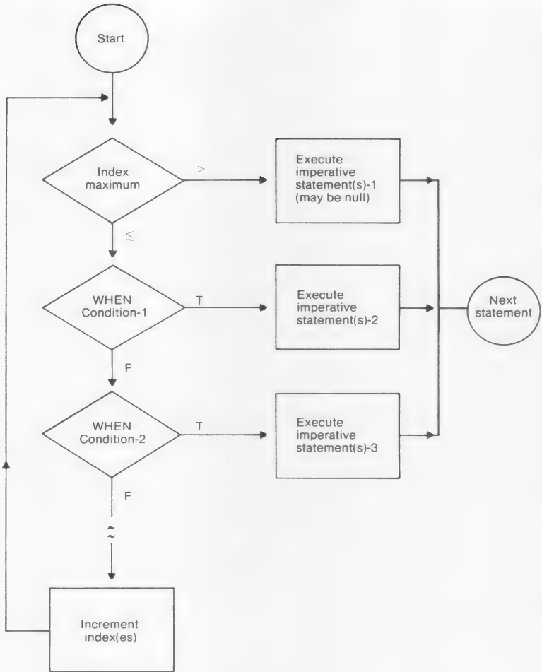
Figure 8.1. Logic Diagram for Format 1 SEARCH Statement
